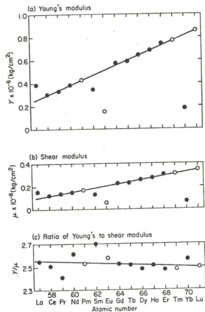
FIG. 2. (a) Young's modulus of the rare-earth metals. (b) Shear modulus of the rare-earth metals. (c) The ratio of Young's modulus to the shear modulus of the rare-earth metals. Open points are estimated values.
